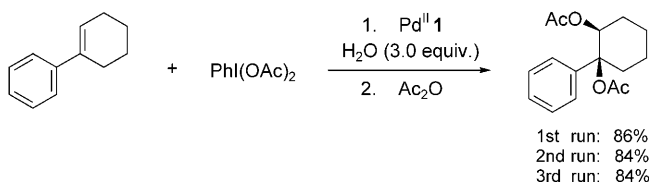
Scheme 2. Stable catalytic activity of the Pd magnetic particles 1 in batch dioxygenation reaction. Standard reaction conditions: 1.65 mol % Pd magnetic particles 1 , DMF/ \text{AcOH} (1:2), 50°C, 5 h. Yields were measured by NMR spectroscopy against an internal standard.
